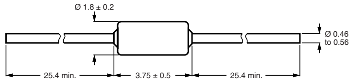
Component outline for 2381 633 8.... (SOD27)
