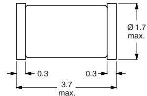
Component outline for 2381 633 5.... (SOD80)
